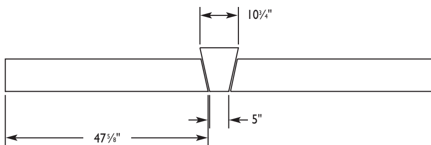
5-Course, (Keystone KY-700)
