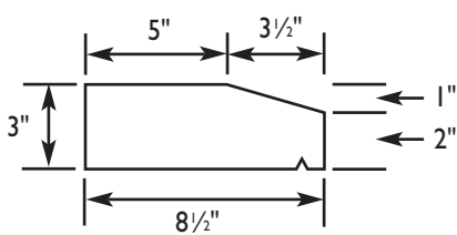
SL-485 (Standard length 35 3/8")
