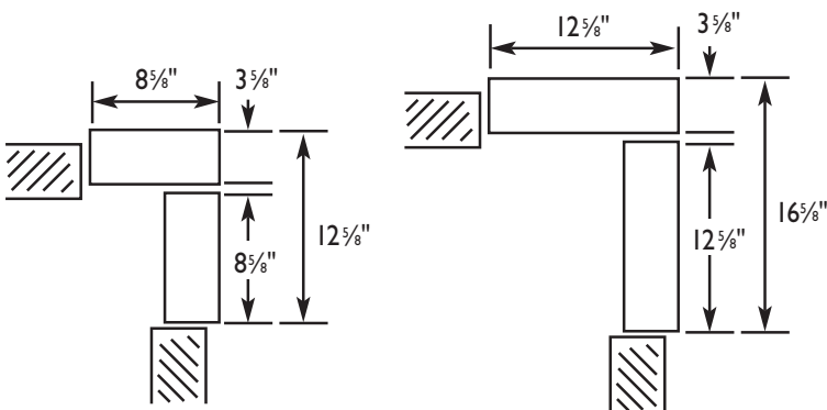
3- and 4-Course Staggered Corners
