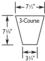
KY-300 Plain KY-310 Chamfered
