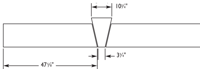
5-Course, (Keystone KY-600)
