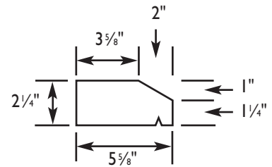
SL-225 (Standard length 23 \frac{3}{8} " )
