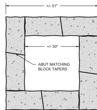
TYPICAL COURSE (PLAN VIEW)
